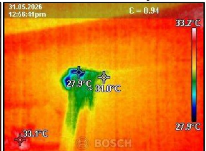
Thermal image of live moisture on ceiling
