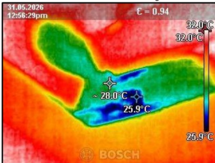
Thermal image of live moisture on ceiling
