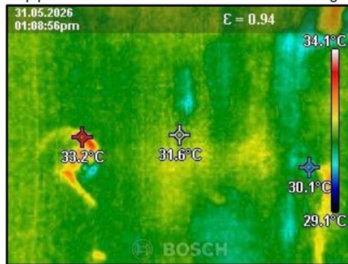
Thermal image of water leakage from pipe line
